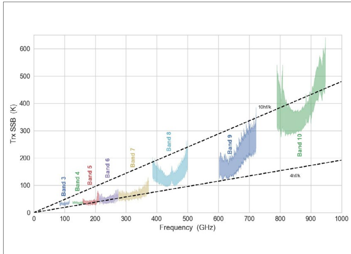
Figure 1: Receiver noise temperature for the ALMA receiver, where the shaded region encompasses 75% of the receivers about the median receiver temperature. Bands 3-8 are 2SB receivers, and Bands 9 and 10 are DSB. The noise temperature shown for the DSB receivers are twice the DSB temperatures. Band 1, which is under construction, has a receiver specification of < 25 K across 80% of the band.
